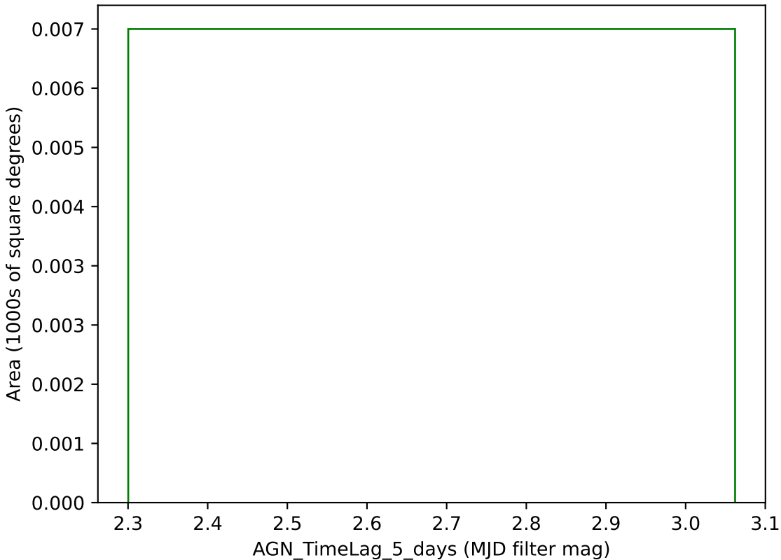
no_high_blob_v3.3_10yrs g band: AGN_TimeLag_5_days
