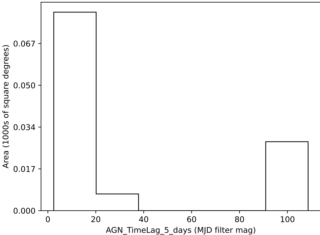
no_high_blob_v3.3_10yrs all bands: AGN_TimeLag_5_days
