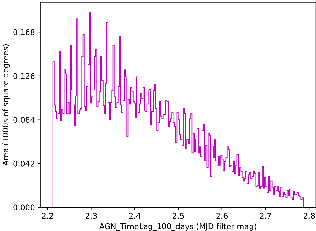
no_high_blob_v3.3_10yrs z band: AGN_TimeLag_100_days
