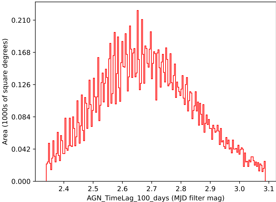
no_high_blob_v3.3_10yrs i band: AGN_TimeLag_100_days
