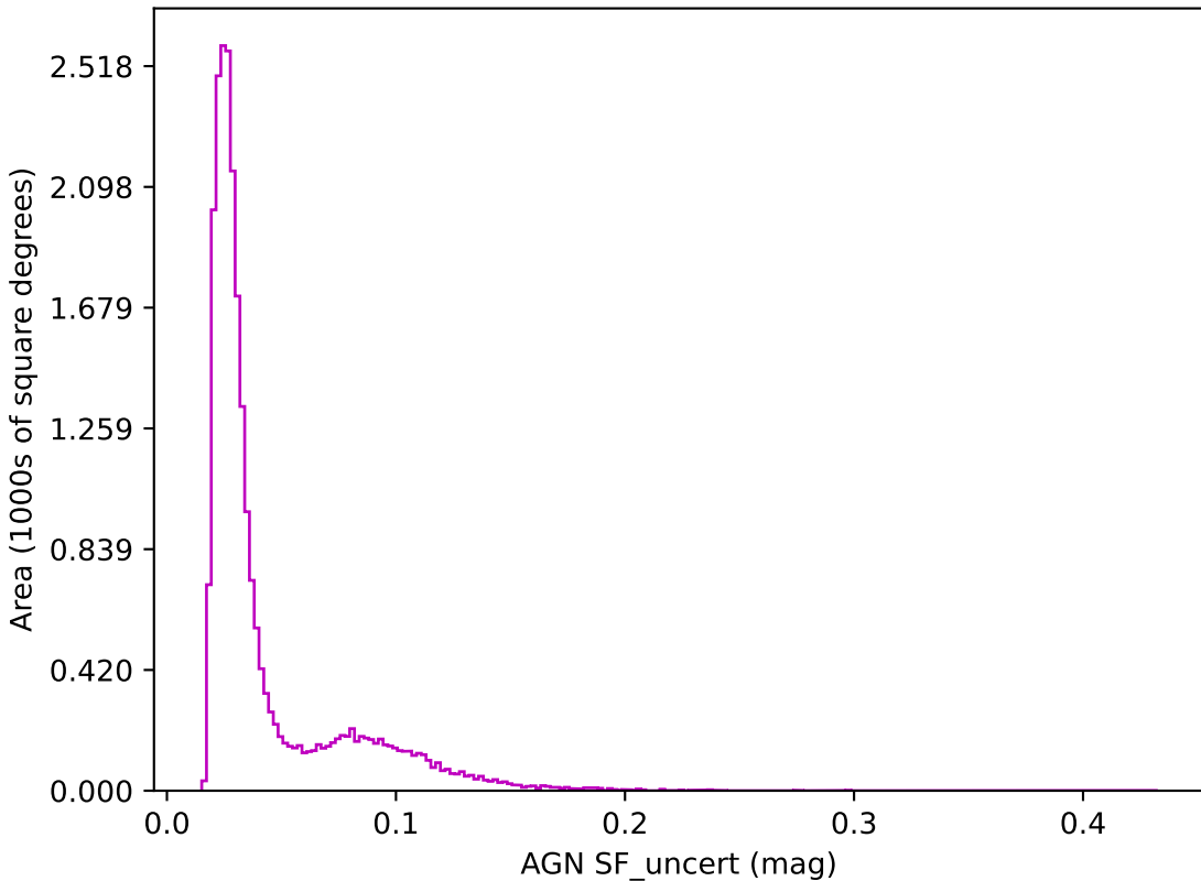
no_high_blob_v3.3_10yrs z band: AGN SF_uncert
