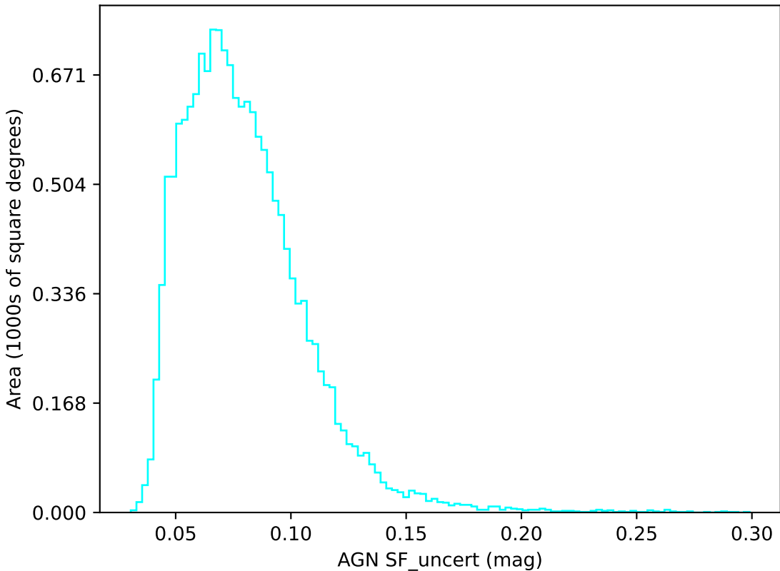
no_high_blob_v3.3_10yrs u band: AGN SF_uncert
