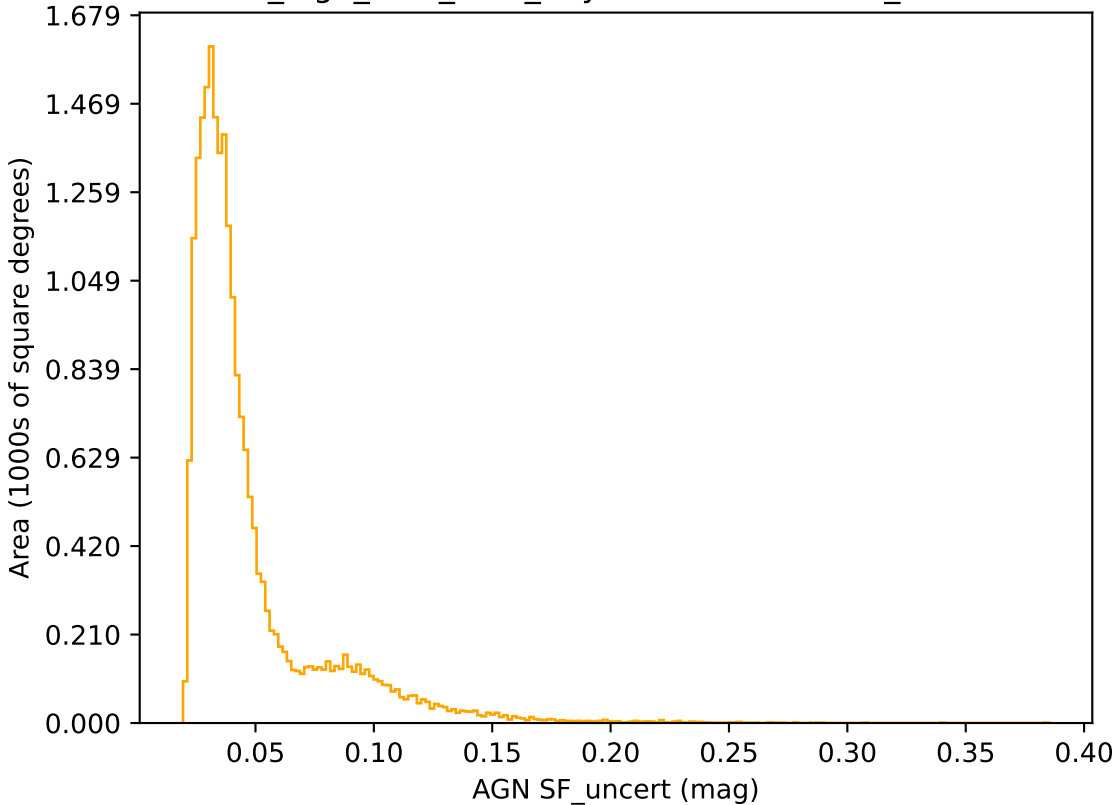
no_high_blob_v3.3_10yrs r band: AGN SF_uncert
