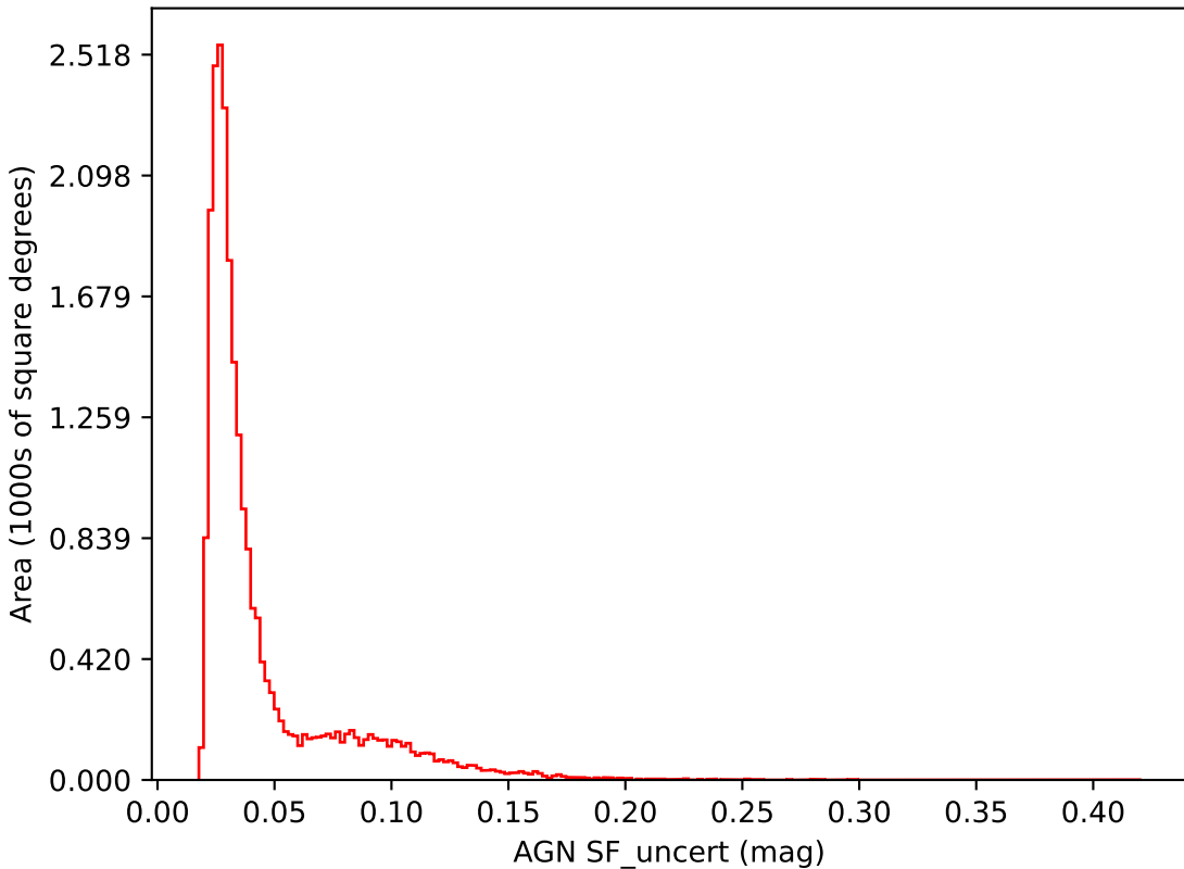
no_high_blob_v3.3_10yrs i band: AGN SF_uncert
