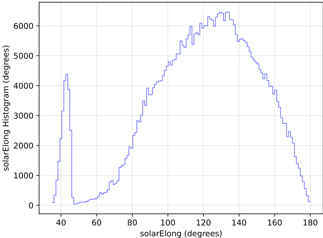
no_high_blob_v3.3_10yrs WFD z band: solarElong Histogram
