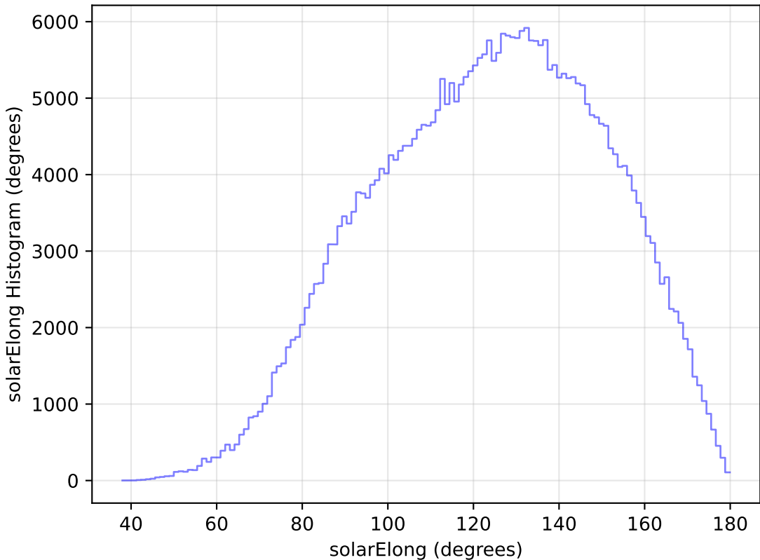
no_high_blob_v3.3_10yrs WFD y band: solarElong Histogram
