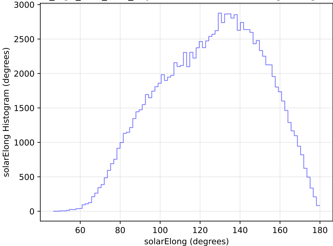
no_high_blob_v3.3_10yrs WFD u band: solarElong Histogram
