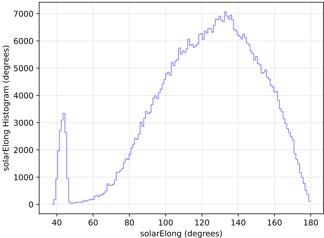
no_high_blob_v3.3_10yrs WFD r band: solarElong Histogram
