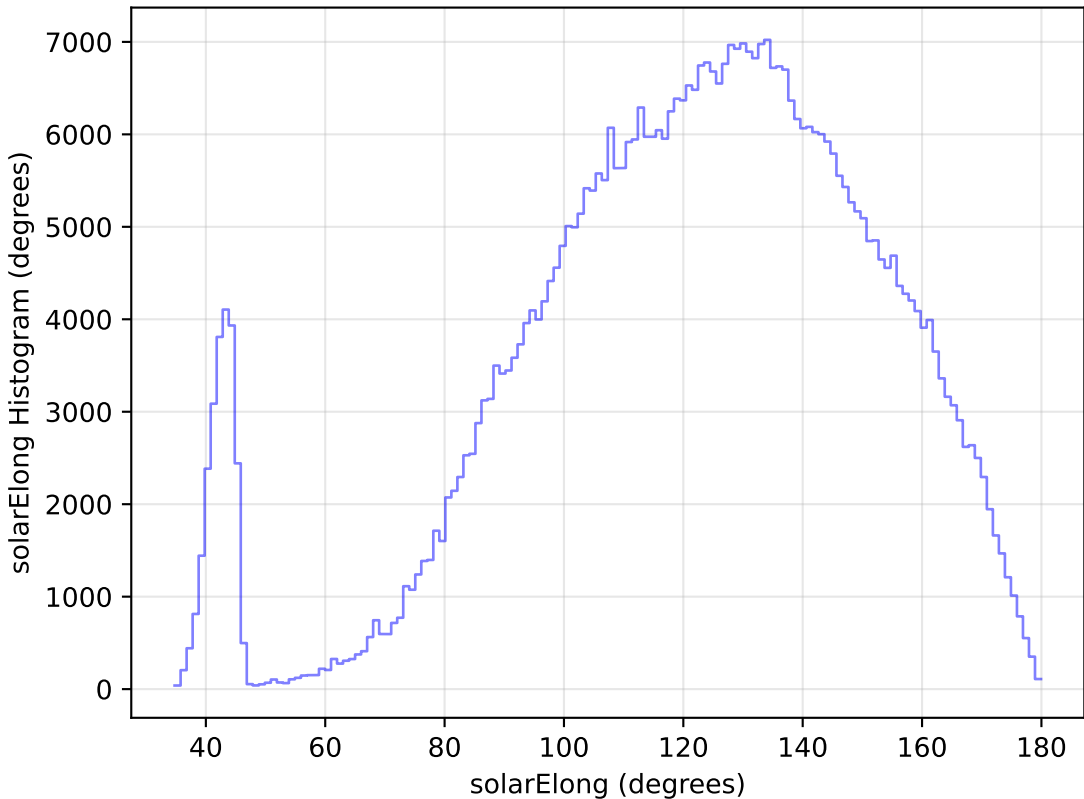
no_high_blob_v3.3_10yrs WFD i band: solarElong Histogram
