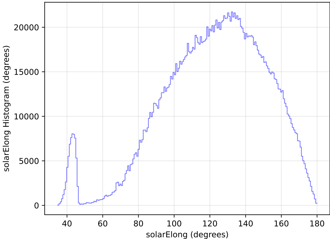
no_high_blob_v3.3_10yrs WFD all bands: solarElong Histogram
