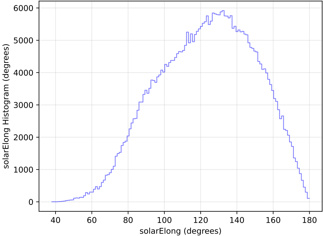
no_high_blob_v3.3_10yrs All sky y band: solarElong Histogram
