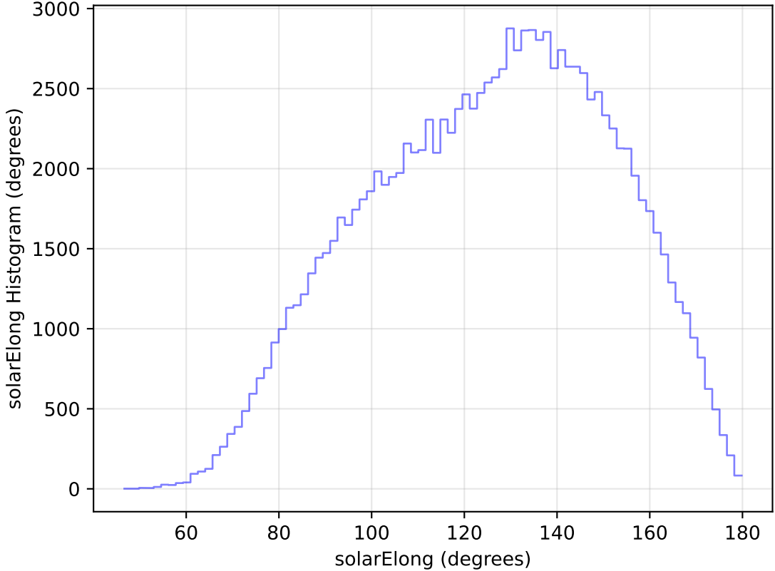
no_high_blob_v3.3_10yrs All sky u band: solarElong Histogram
