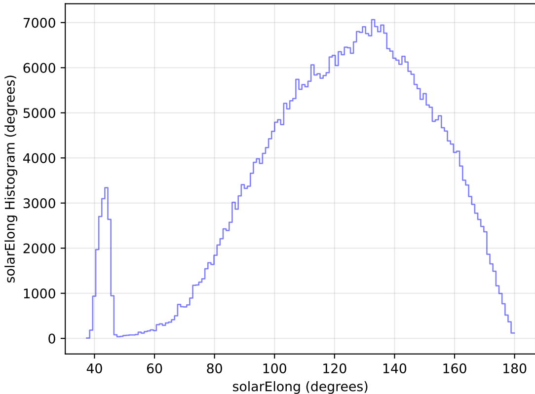
no_high_blob_v3.3_10yrs All sky r band: solarElong Histogram
