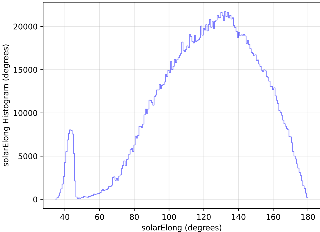
no_high_blob_v3.3_10yrs All sky all bands: solarElong Histogram
