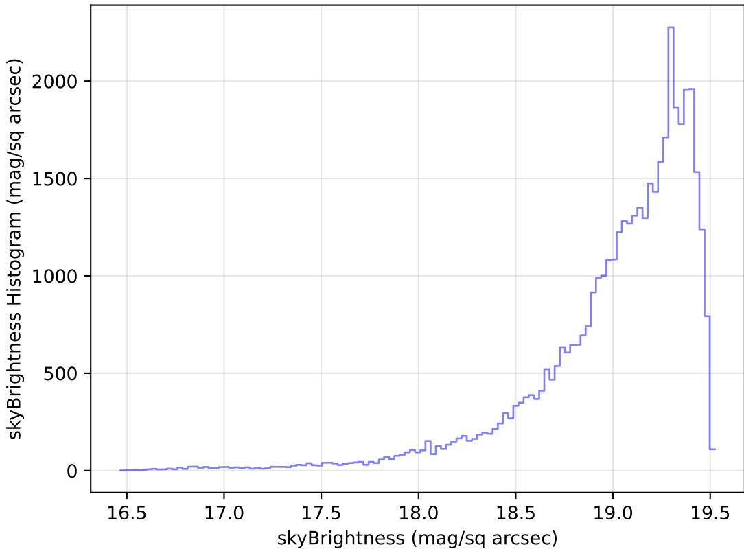
no_high_blob_v3.3_10yrs Yr 1 z band: skyBrightness Histogram
