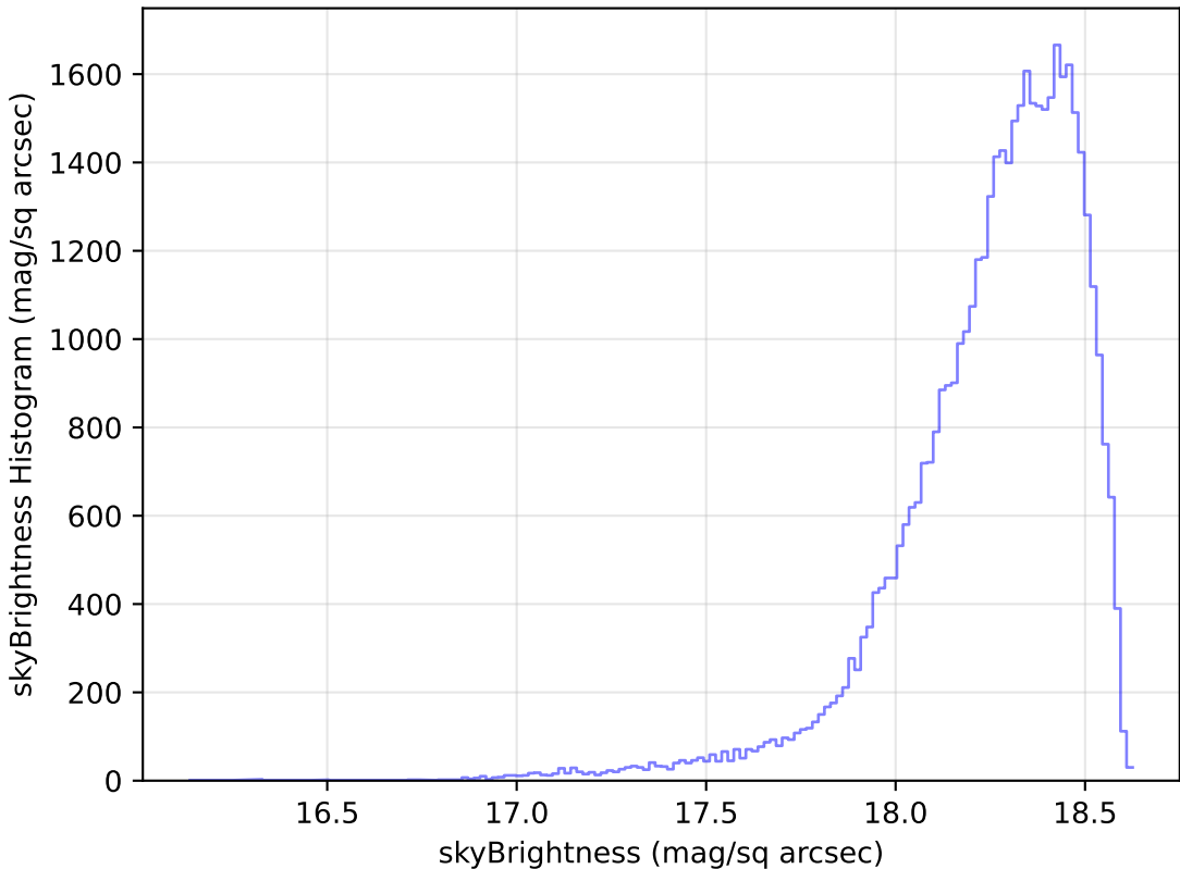
no_high_blob_v3.3_10yrs Yr 1 y band: skyBrightness Histogram
