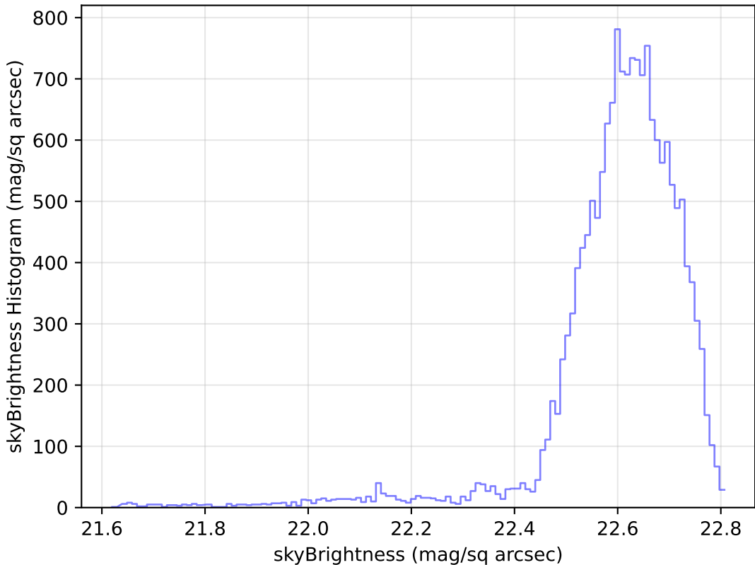
no_high_blob_v3.3_10yrs Yr 1 u band: skyBrightness Histogram
