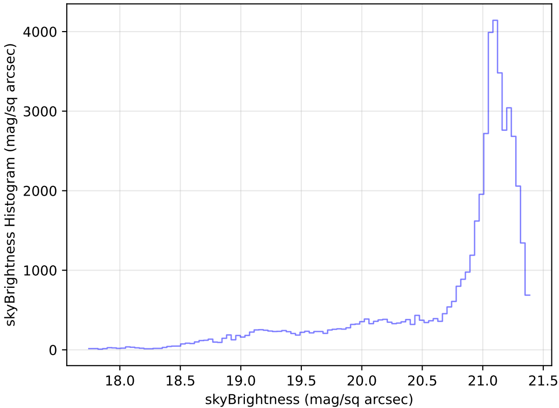
no_high_blob_v3.3_10yrs Yr 1 r band: skyBrightness Histogram
