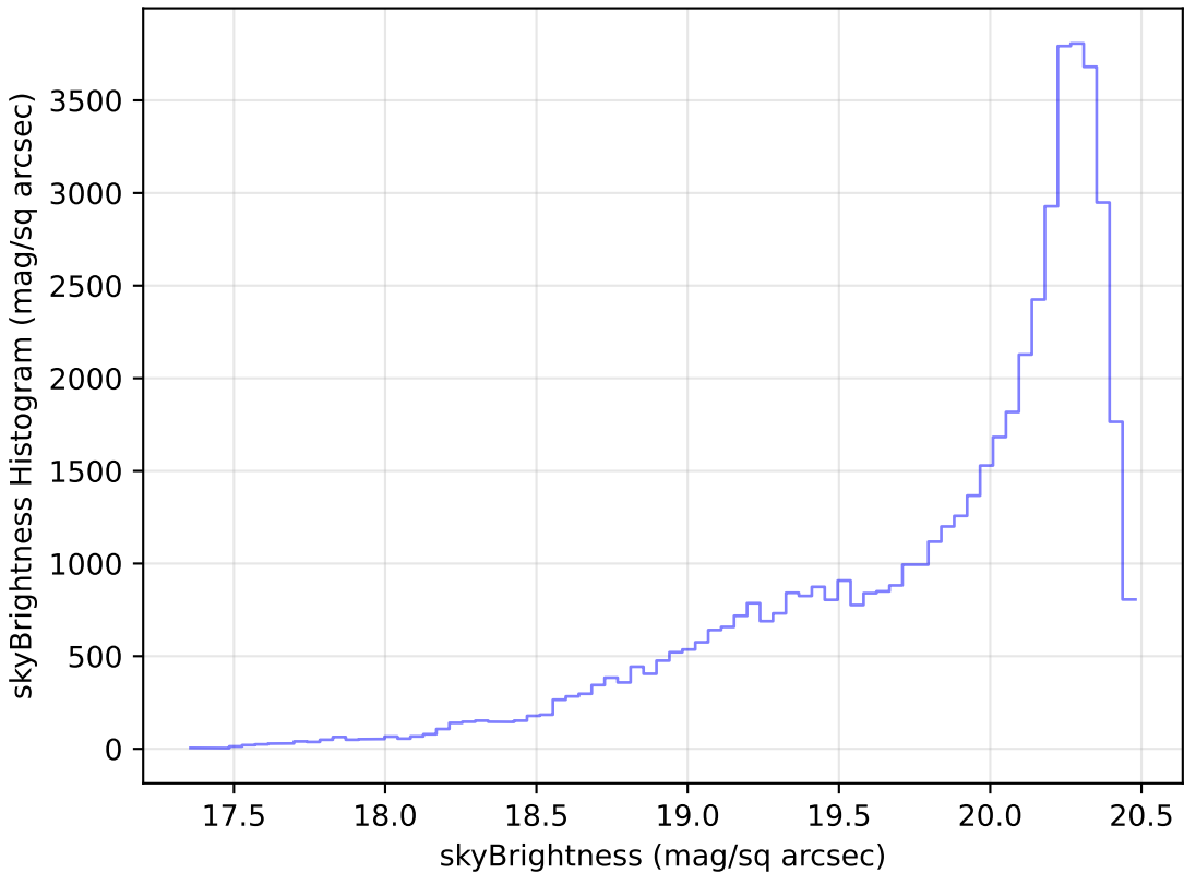
no_high_blob_v3.3_10yrs Yr 1 i band: skyBrightness Histogram
