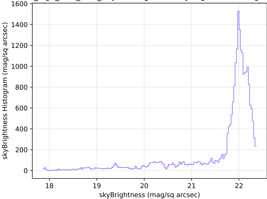
no_high_blob_v3.3_10yrs Yr 1 g band: skyBrightness Histogram
