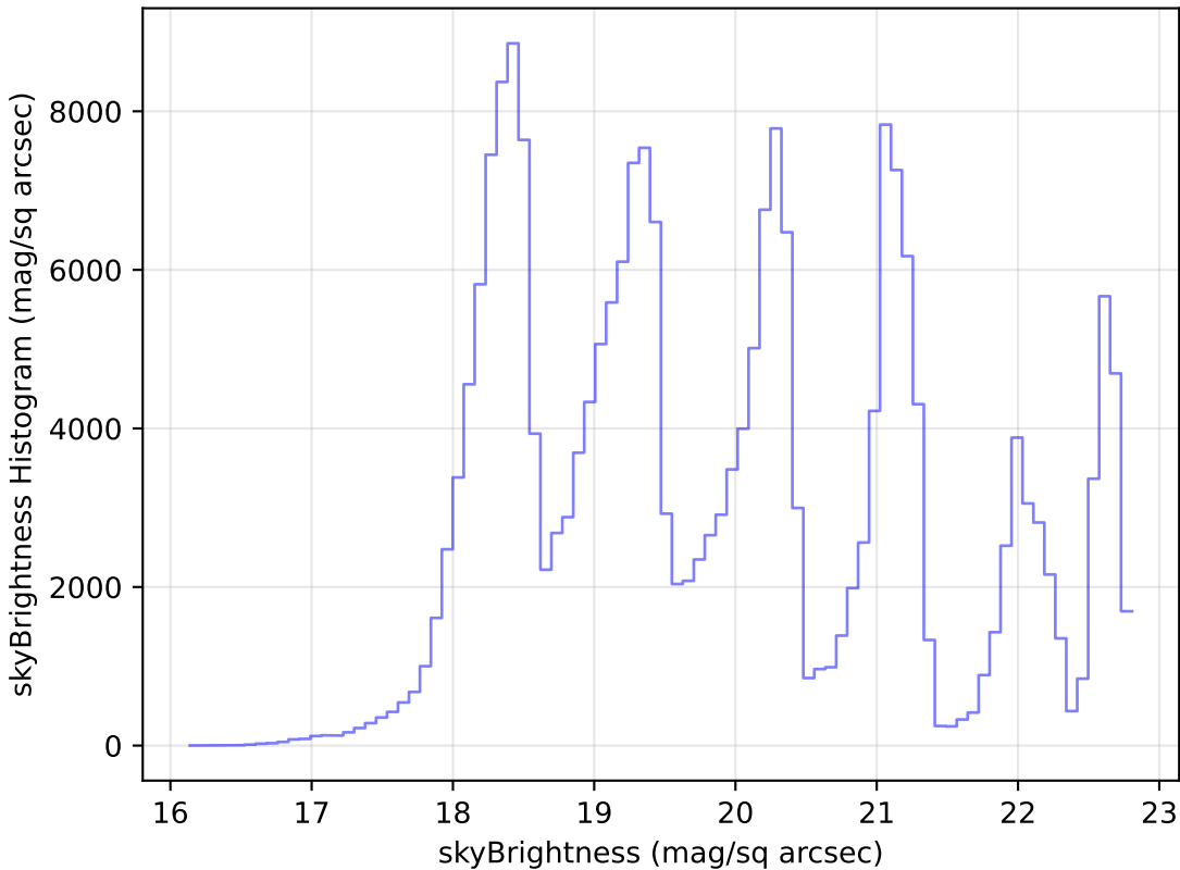
no_high_blob_v3.3_10yrs Yr 1 all bands: skyBrightness Histogram
