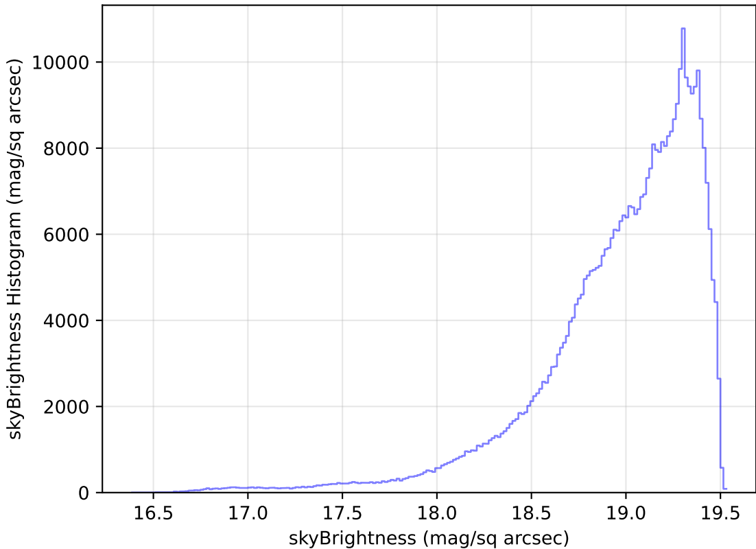
no_high_blob_v3.3_10yrs WFD z band: skyBrightness Histogram
