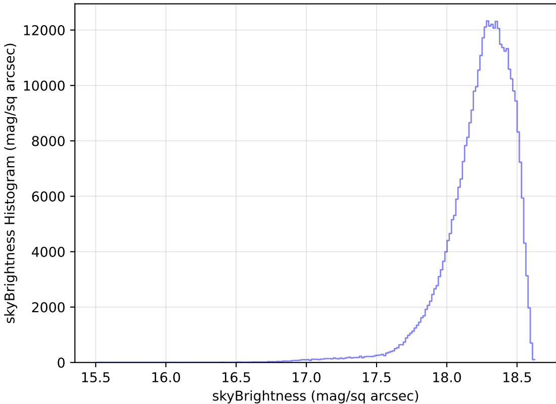
no_high_blob_v3.3_10yrs WFD y band: skyBrightness Histogram
