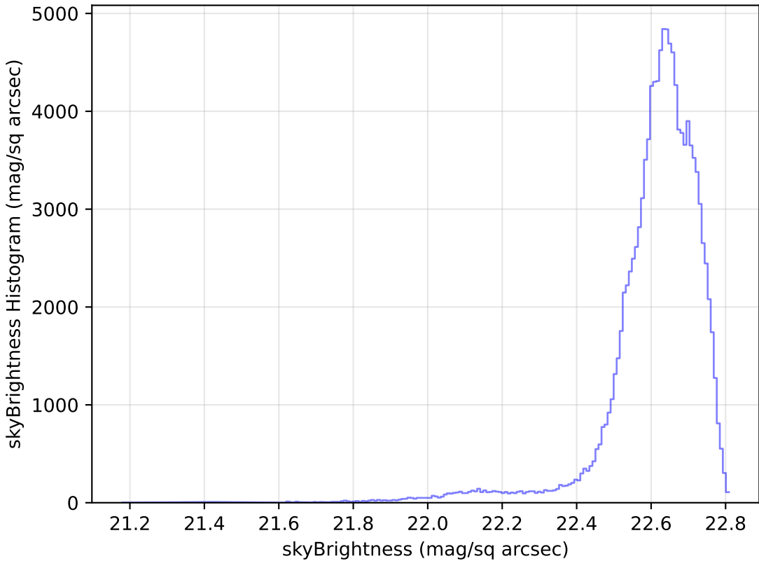
no_high_blob_v3.3_10yrs WFD u band: skyBrightness Histogram
