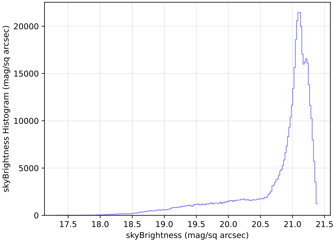
no_high_blob_v3.3_10yrs WFD r band: skyBrightness Histogram
