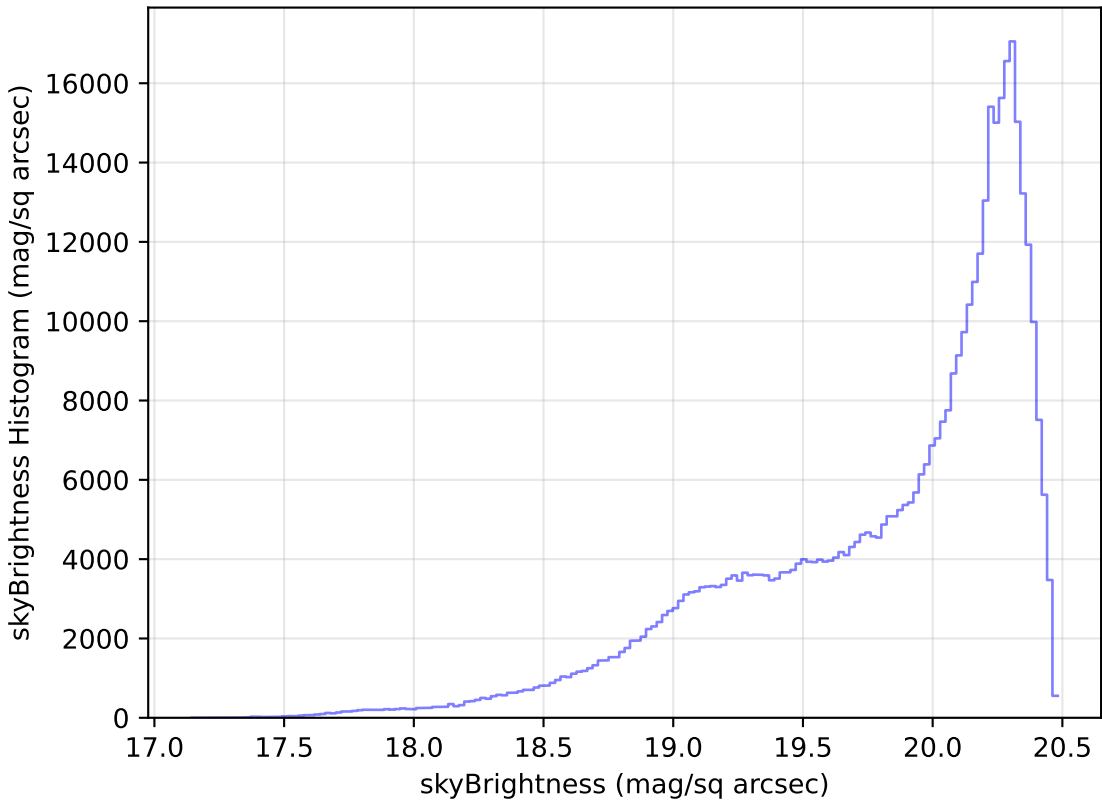
no_high_blob_v3.3_10yrs WFD i band: skyBrightness Histogram
