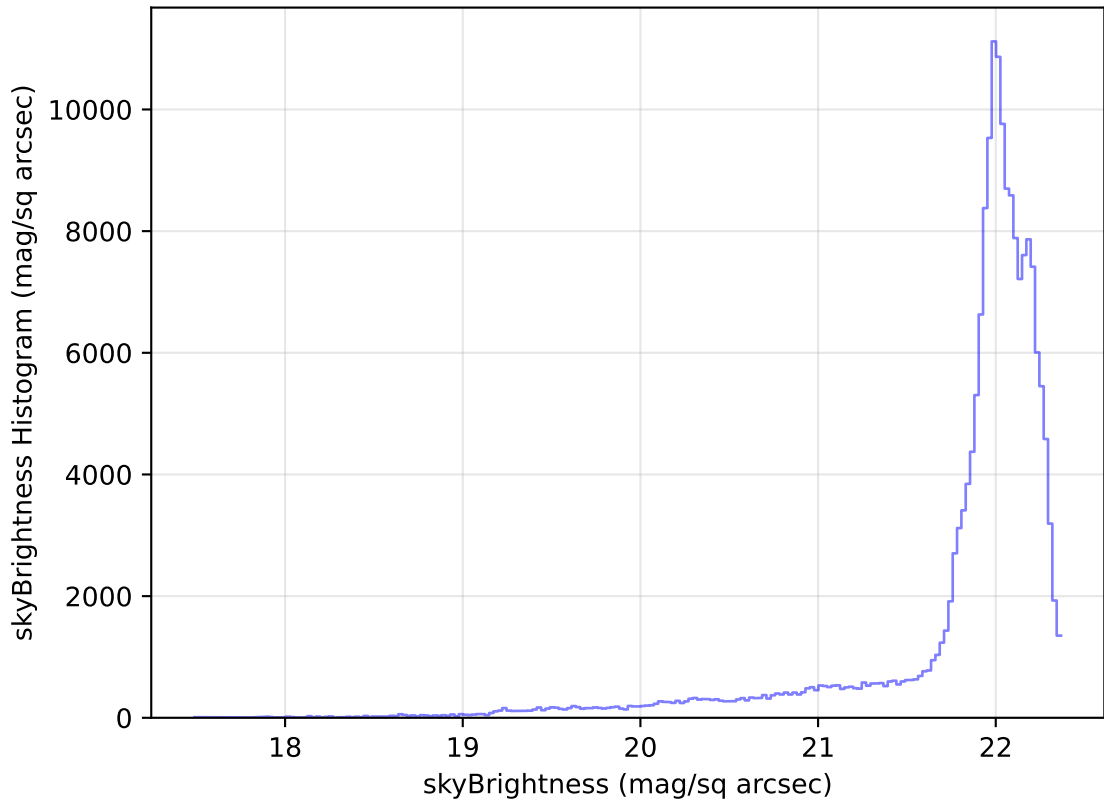
no_high_blob_v3.3_10yrs WFD g band: skyBrightness Histogram
