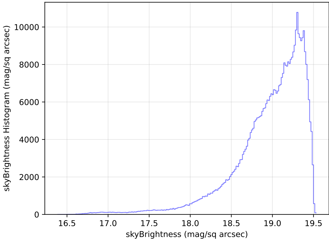
no_high_blob_v3.3_10yrs All sky z band: skyBrightness Histogram
