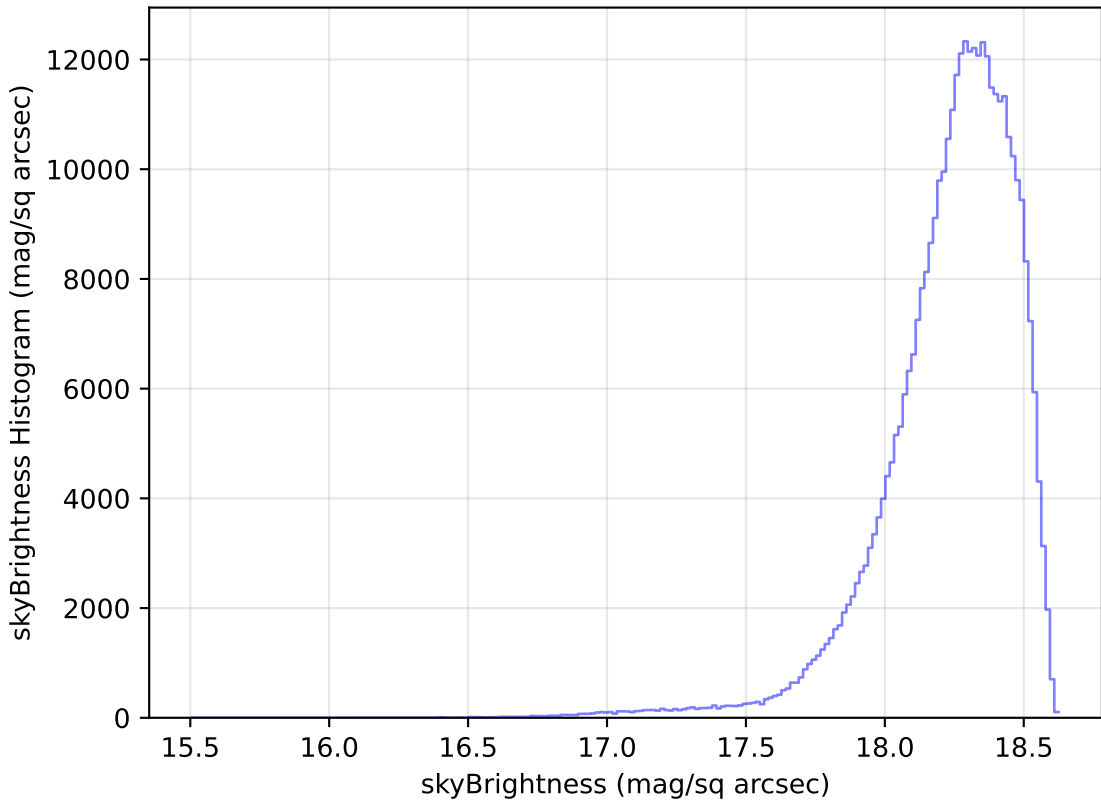
no_high_blob_v3.3_10yrs All sky y band: skyBrightness Histogram
