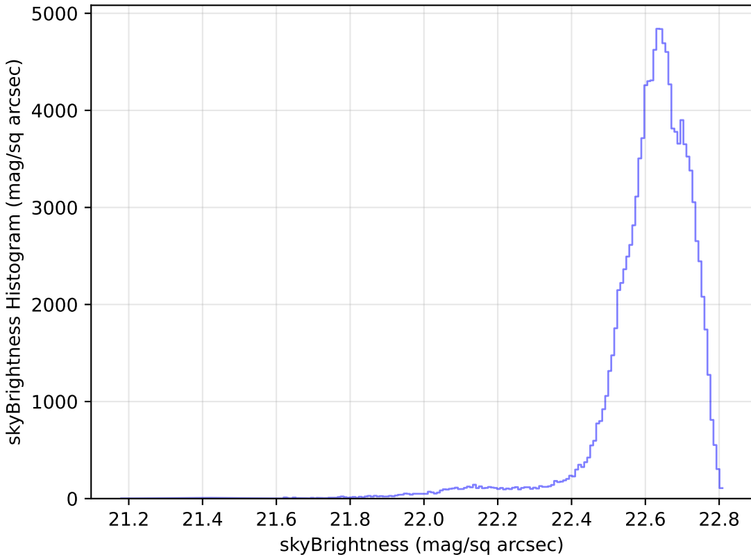
no_high_blob_v3.3_10yrs All sky u band: skyBrightness Histogram
