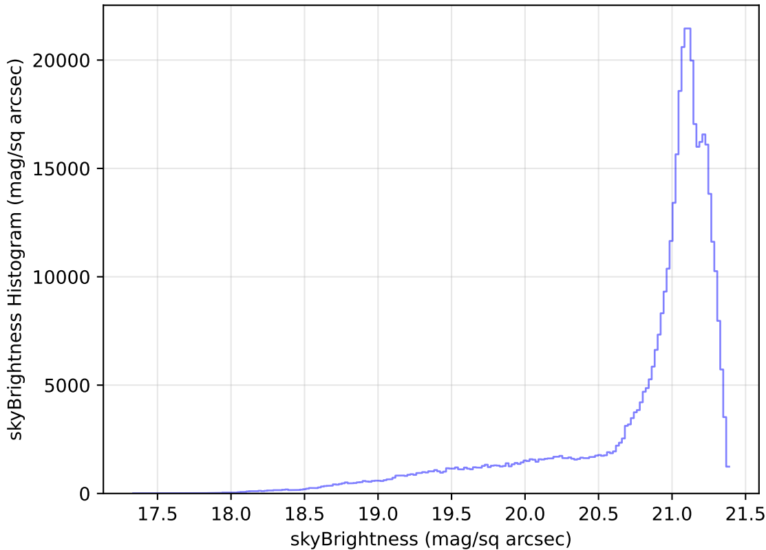
no_high_blob_v3.3_10yrs All sky r band: skyBrightness Histogram
