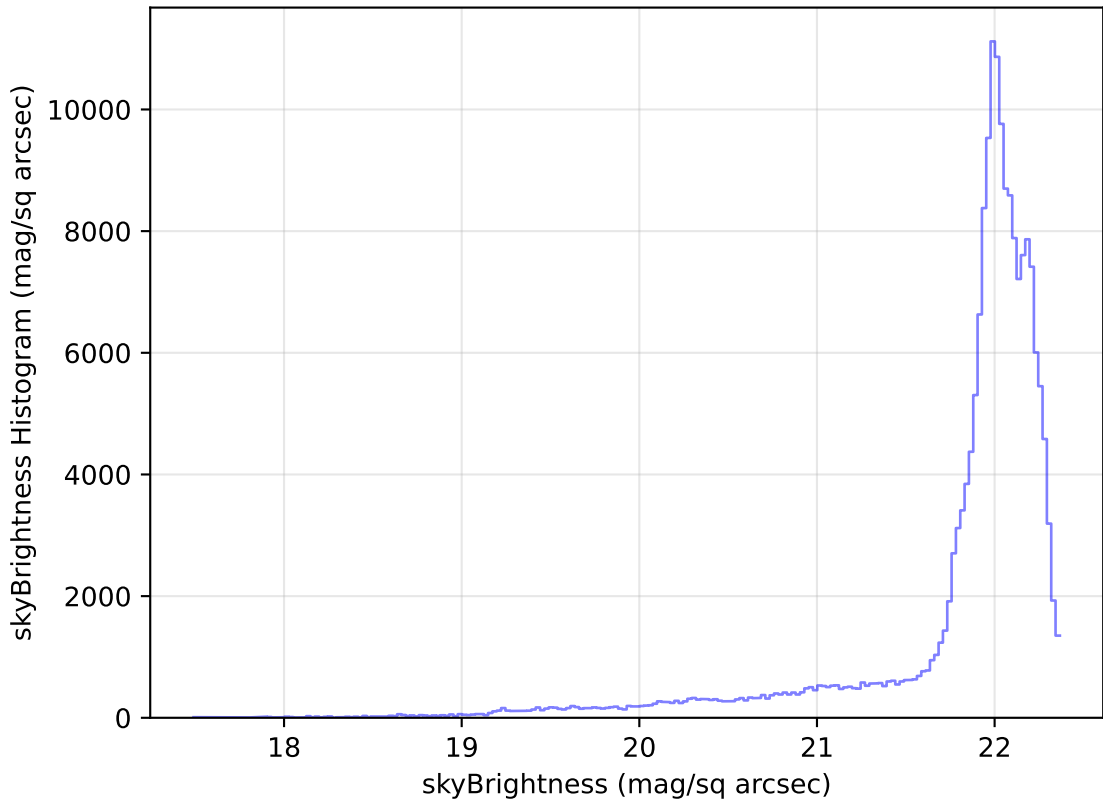
no_high_blob_v3.3_10yrs All sky g band: skyBrightness Histogram
