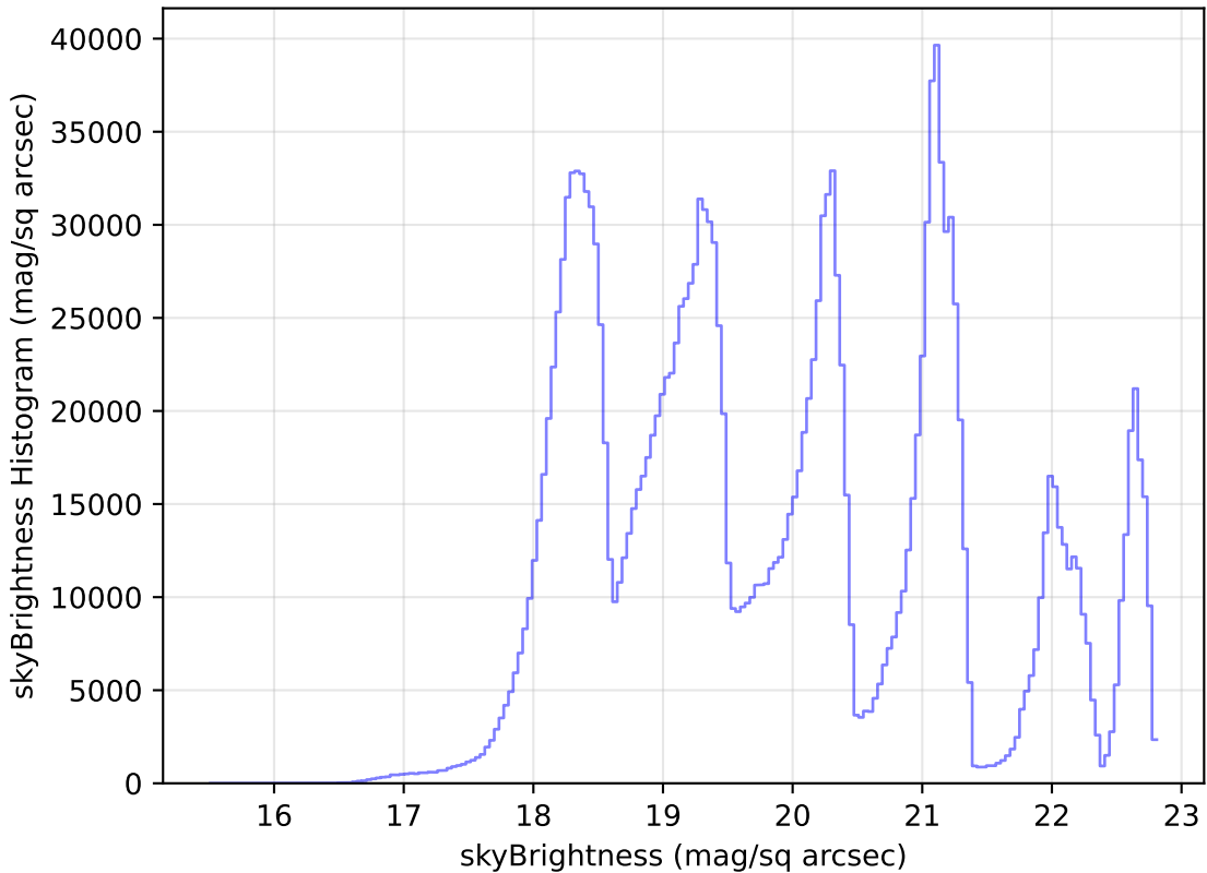
no_high_blob_v3.3_10yrs All sky all bands: skyBrightness Histogram
