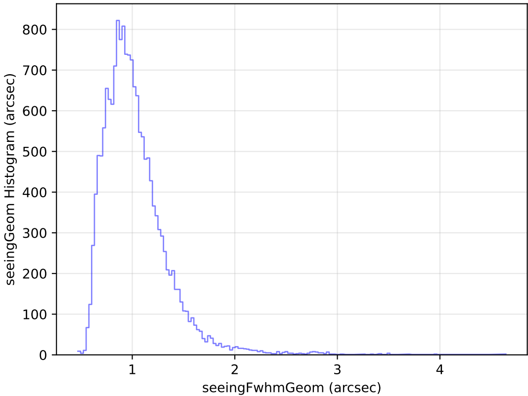
no_high_blob_v3.3_10yrs Yr 1 u band: seeingGeom Histogram
