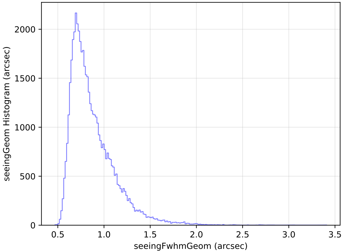
no_high_blob_v3.3_10yrs Yr 1 r band: seeingGeom Histogram
