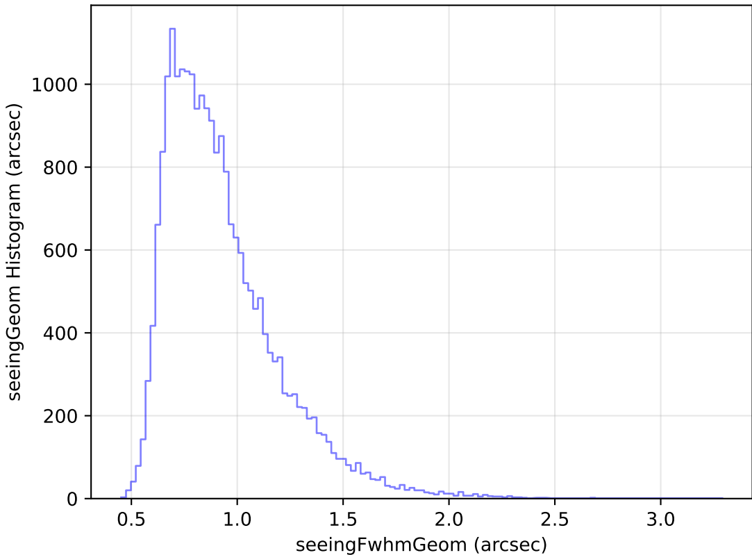
no_high_blob_v3.3_10yrs Yr 1 g band: seeingGeom Histogram
