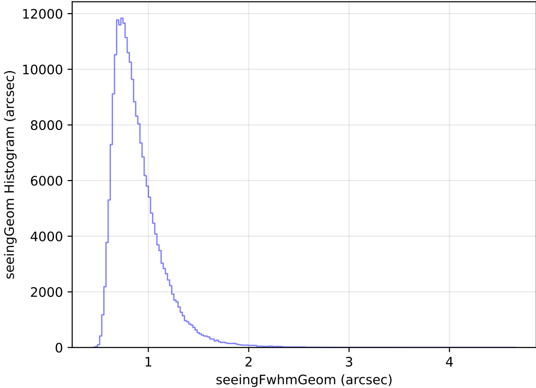
no_high_blob_v3.3_10yrs Yr 1 all bands: seeingGeom Histogram
