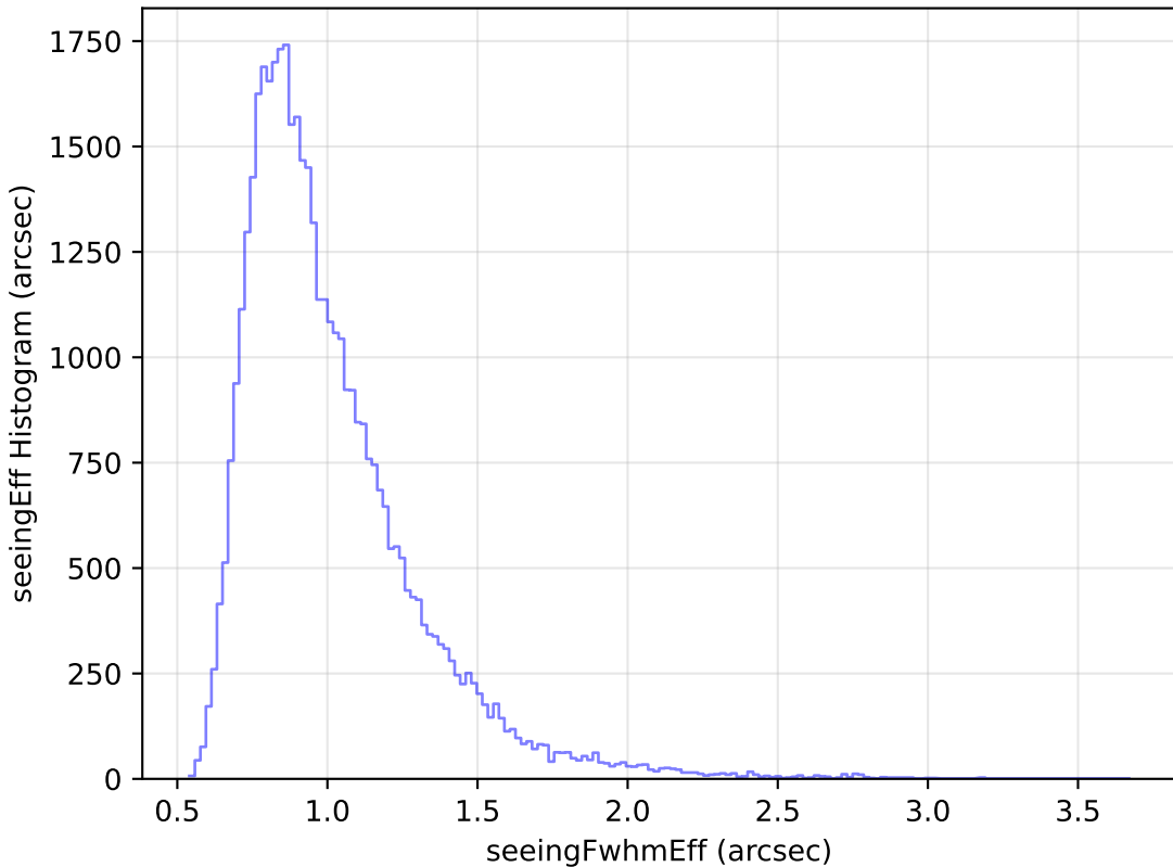
no_high_blob_v3.3_10yrs Yr 1 z band: seeingEff Histogram
