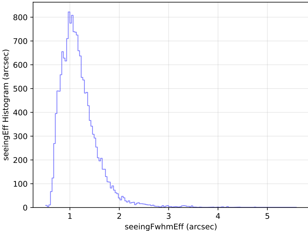
no_high_blob_v3.3_10yrs Yr 1 u band: seeingEff Histogram
