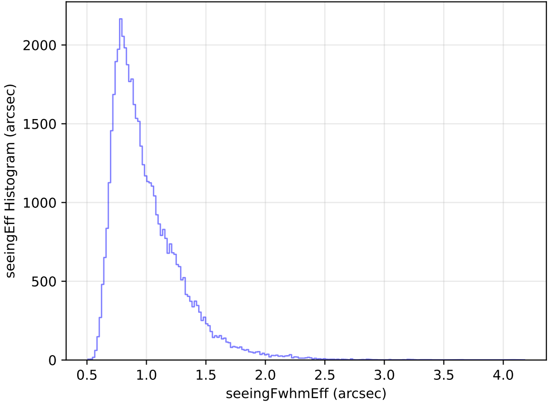
no_high_blob_v3.3_10yrs Yr 1 r band: seeingEff Histogram
