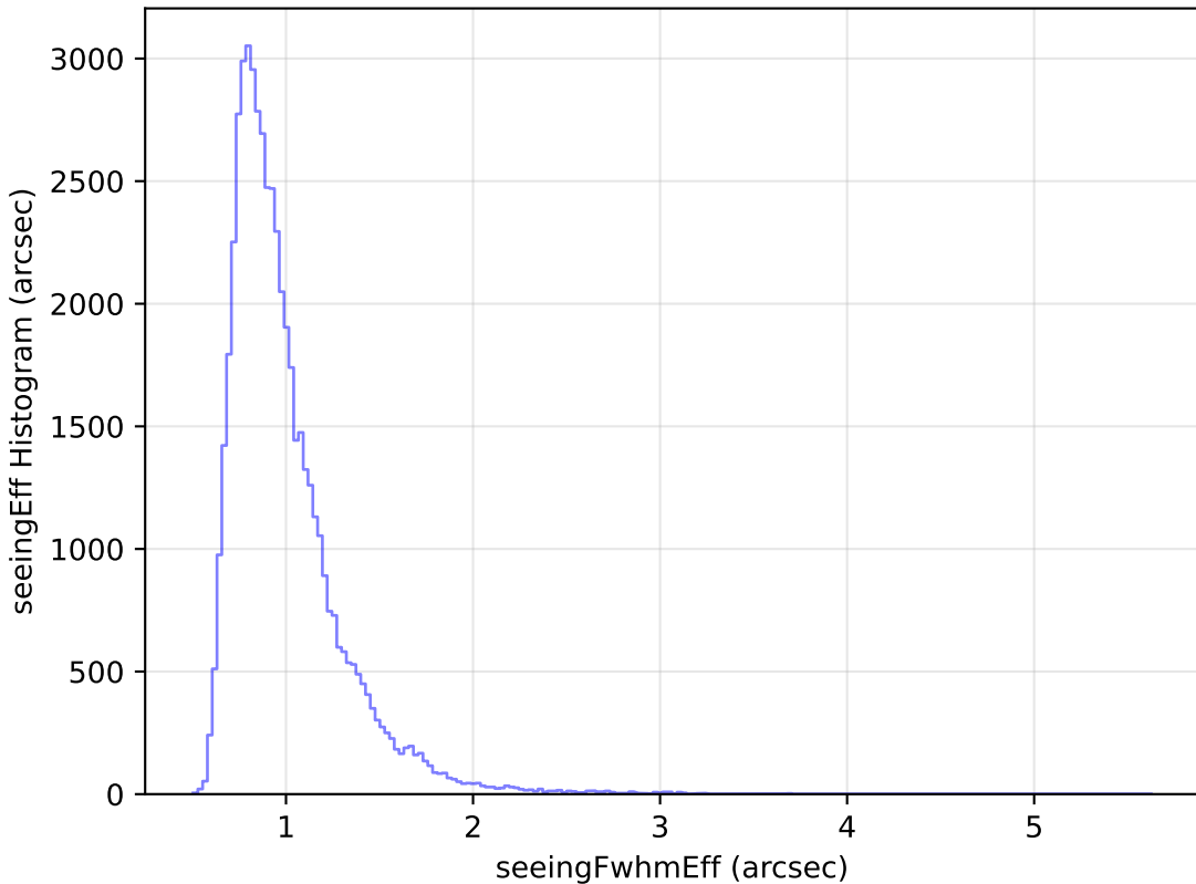
no_high_blob_v3.3_10yrs Yr 1 i band: seeingEff Histogram
