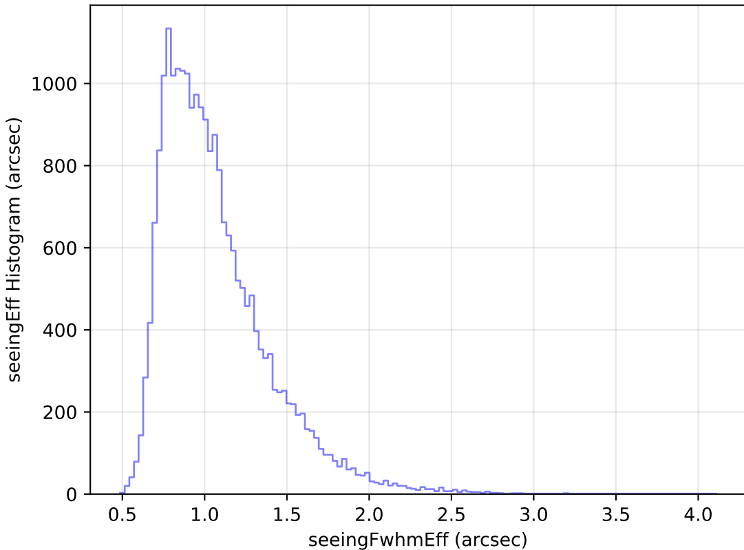
no_high_blob_v3.3_10yrs Yr 1 g band: seeingEff Histogram
