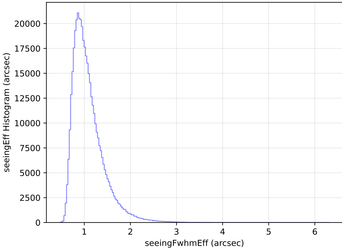
no_high_blob_v3.3_10yrs WFD z band: seeingEff Histogram
