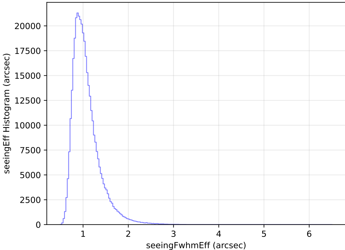
no_high_blob_v3.3_10yrs WFD y band: seeingEff Histogram
