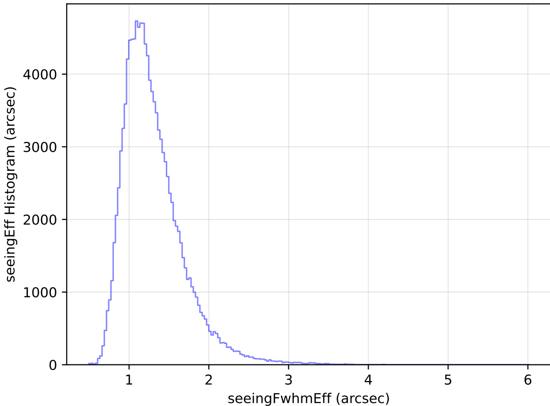
no_high_blob_v3.3_10yrs WFD u band: seeingEff Histogram
