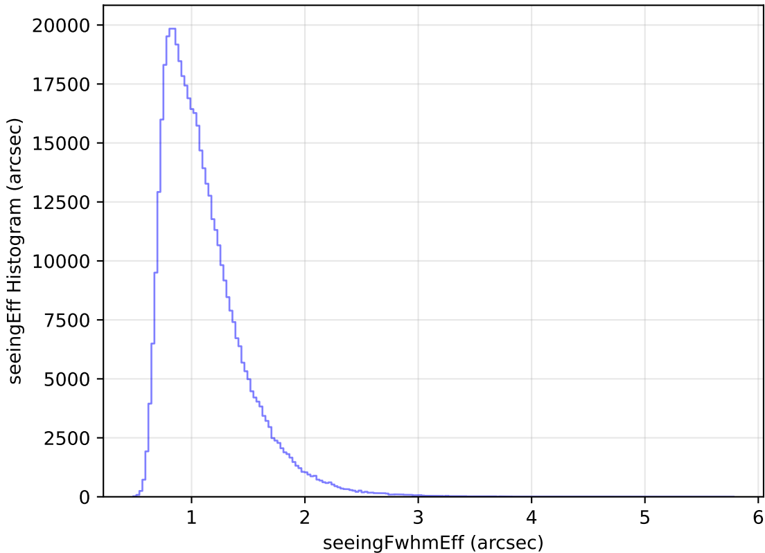
no_high_blob_v3.3_10yrs WFD r band: seeingEff Histogram
